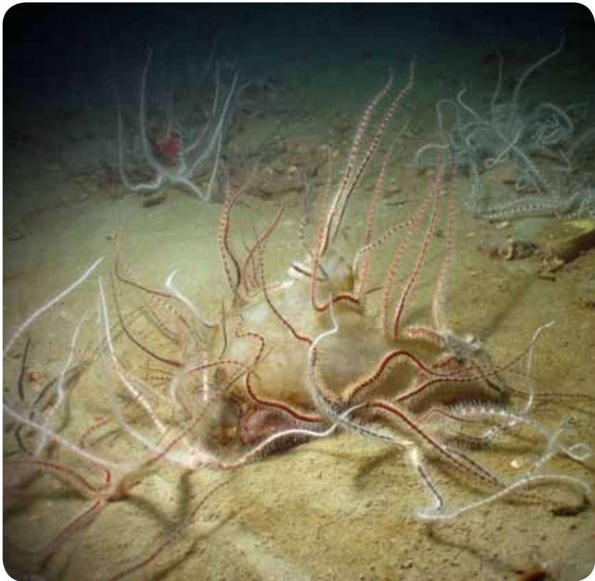
Figure 13: Clusters of benthic organisms in coastal detritic bottom biocoenoses.
