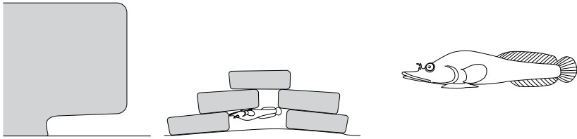
Figure 61: Real cryptobenthic species and their microhabitat.
