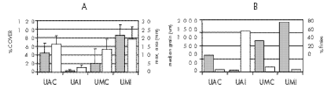
Figure 2. A) Mean rhodolith cover and length of maximum axis of living rhodoliths at each locality. B) Median grain size and percentage of fines (<63 μm) at each locality. (Gray and white bars correspond to left and right scales respectively; error bars are +1SD).
