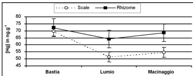
Fig. 2: Mercury concentration (in \text{ng.g}^{-1} dry weight) in scales and rhizomes of Posidonia oceanica in function of the site, all years mingled.
