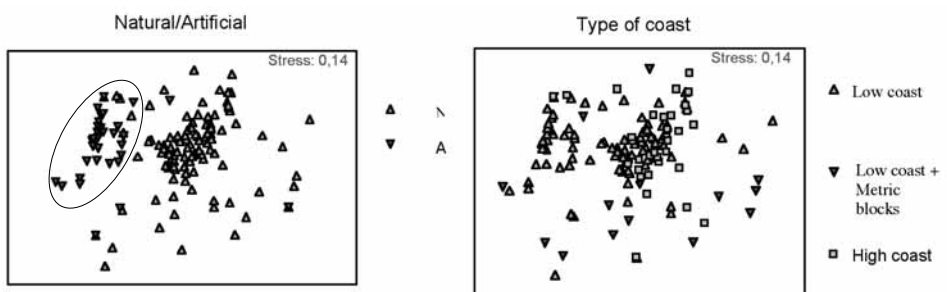
Fig. 1 : MDS analysis: distribution of the 174 different situations resulting from all the available combinations of the geomorphological variables considered in reference sites according to the percentage of coast occupied by each community for each situation. Artificial and natural substrates are indicated with different symbols.
