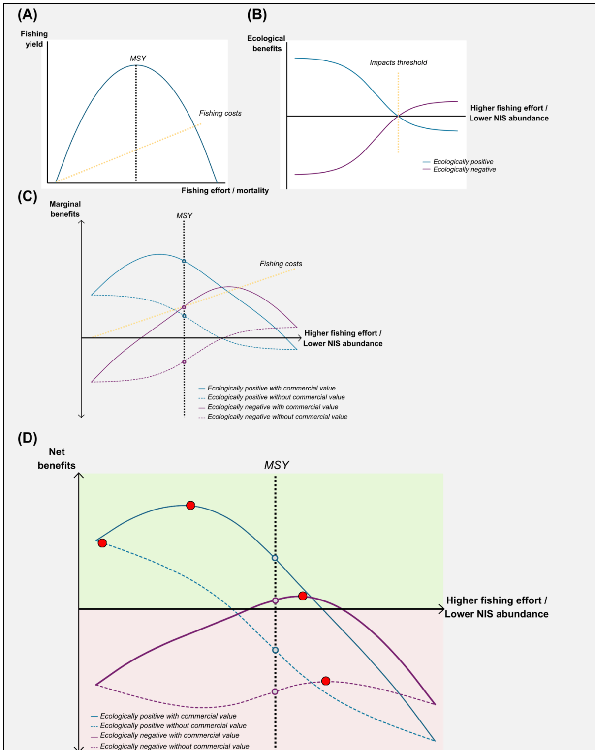
Figure 10. 5A: Relationship between fishing effort and yield, showing the parabolic curve that peaks at the Maximum Sustainable Yield (MSY) and declines with increased effort; 5B: Inverse logistic curves based on the logistic growth theory, demonstrating how ecological benefits vary with fishing efforts, increasing against harmful NIS and decreasing when beneficial NIS are impacted; 5C: Integration of yield data and ecological impacts to assess overall marginal benefits from varied fishing efforts; 5D: Expansion to include fishing costs and the categorization of species by ecological impact and commercial value, highlighting the optimization of net benefits through strategic fishing practices.
