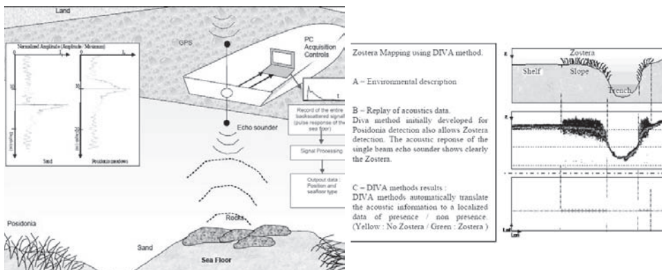
Fig. 6: Left : Principle of DIVA method. In box : Representatives echoes.- Right : Illustration of DIVA approach in Zosteria mapping.
