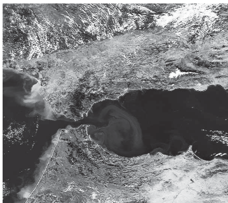
Fig. 1 (see color plate p. 76): Strait of Gibraltar and Western Alboran Sea. Atlantic water (AW) generates strong eddies as passes trough the Strait of Gibraltar. AW undergoes intense mixing causing a loss in heat before it reaches the Alboran Sea. Here upwellings are set mainly on the Spanish side, while clockwise (anticyclonic) eddies generate convergence (downwelling) off the African coast. Image SeaWiFS (S1997361123941.png) http://visibleearth.nasa.gov
